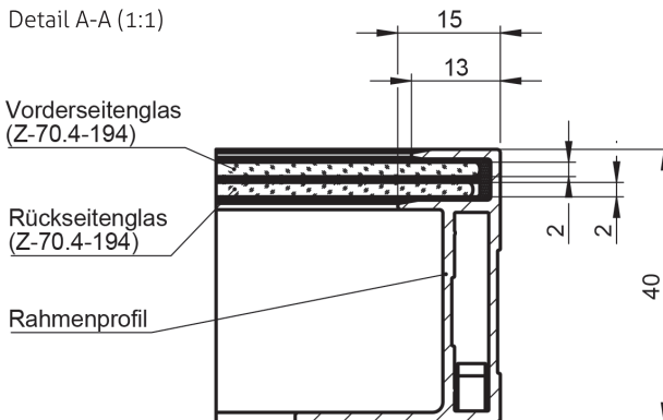
Detail A-A (1:1)
